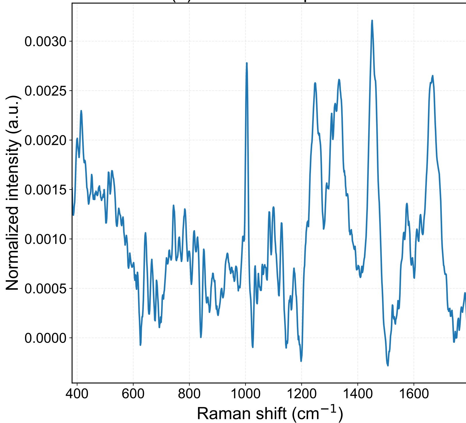
(a) 1D Raman Spectrum
