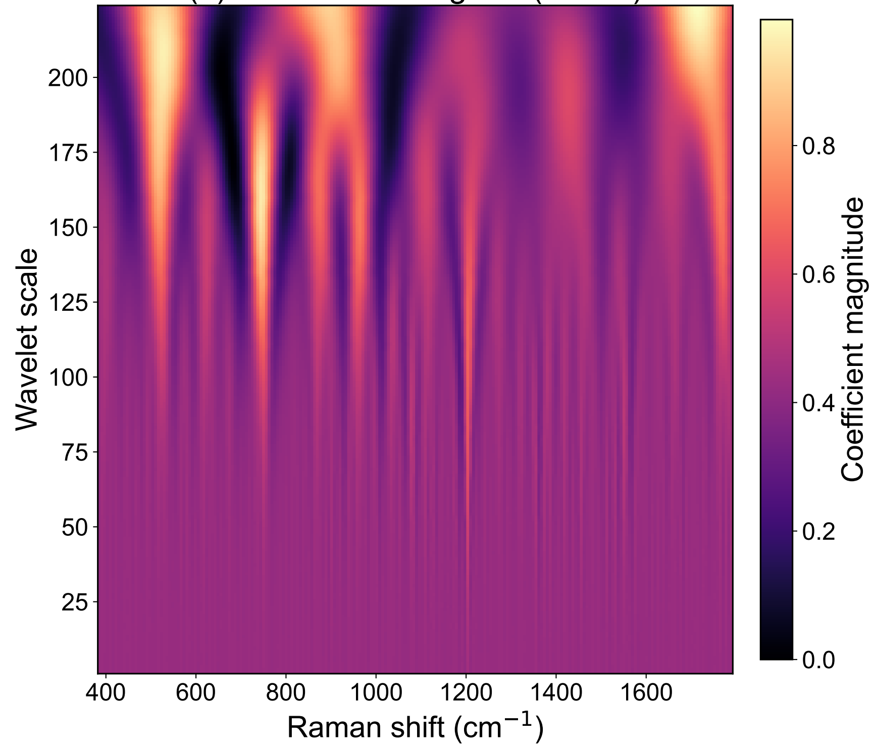
(b) 2D CWT Scalogram (Morlet)
